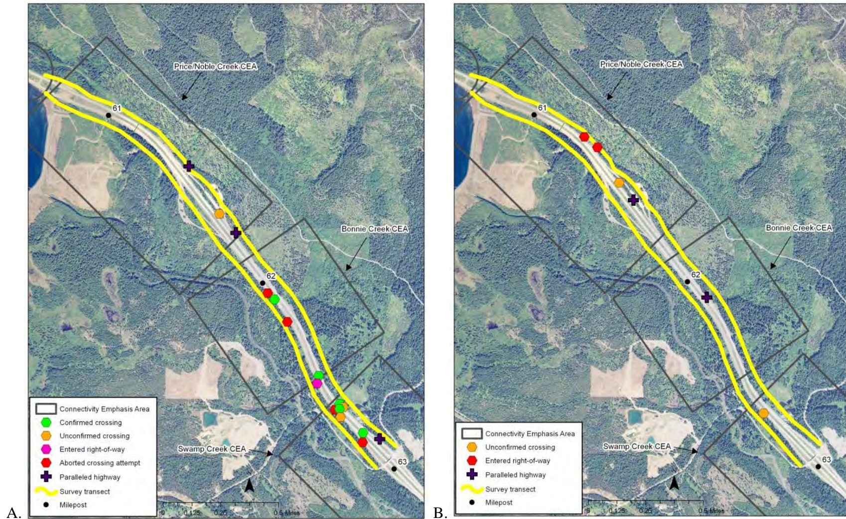
Figure 3.16. Winter 2008–2009 snow track detections, including encounter type, along the Swamp-Bonnie-Price Creek Transect for (A) coyotes and (B) bobcats.
