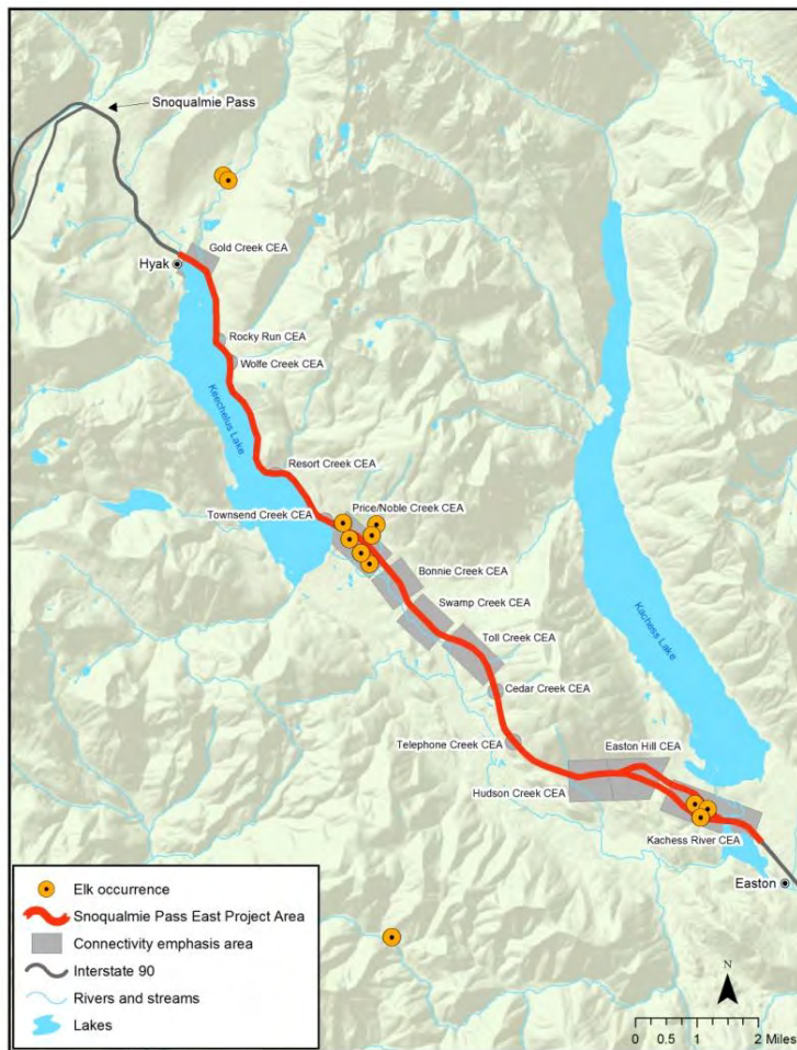
Figure 4.13. Locations where elk were detected by remote camera photographs.
