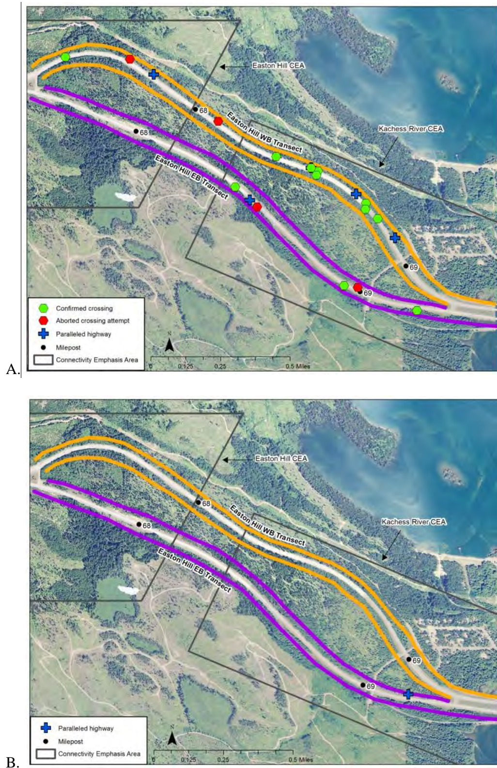
Figure 3.18. Winter 2008–2009 snow track detections, including encounter type, along the Easton Hill WB and EB Transects for (A) coyotes and (B) bobcats.
