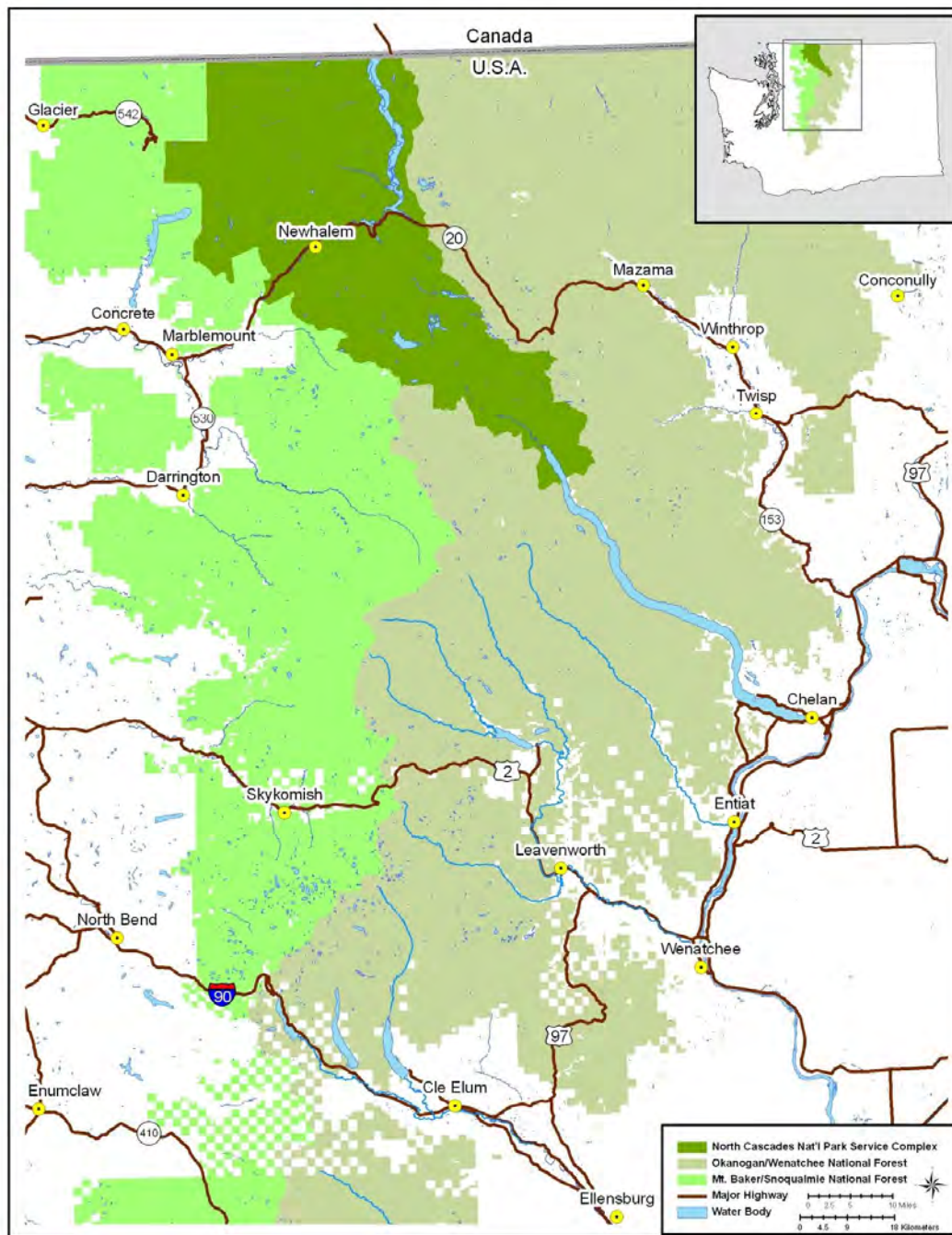
Figure 1. Washington's North Cascades Ecosystem.
