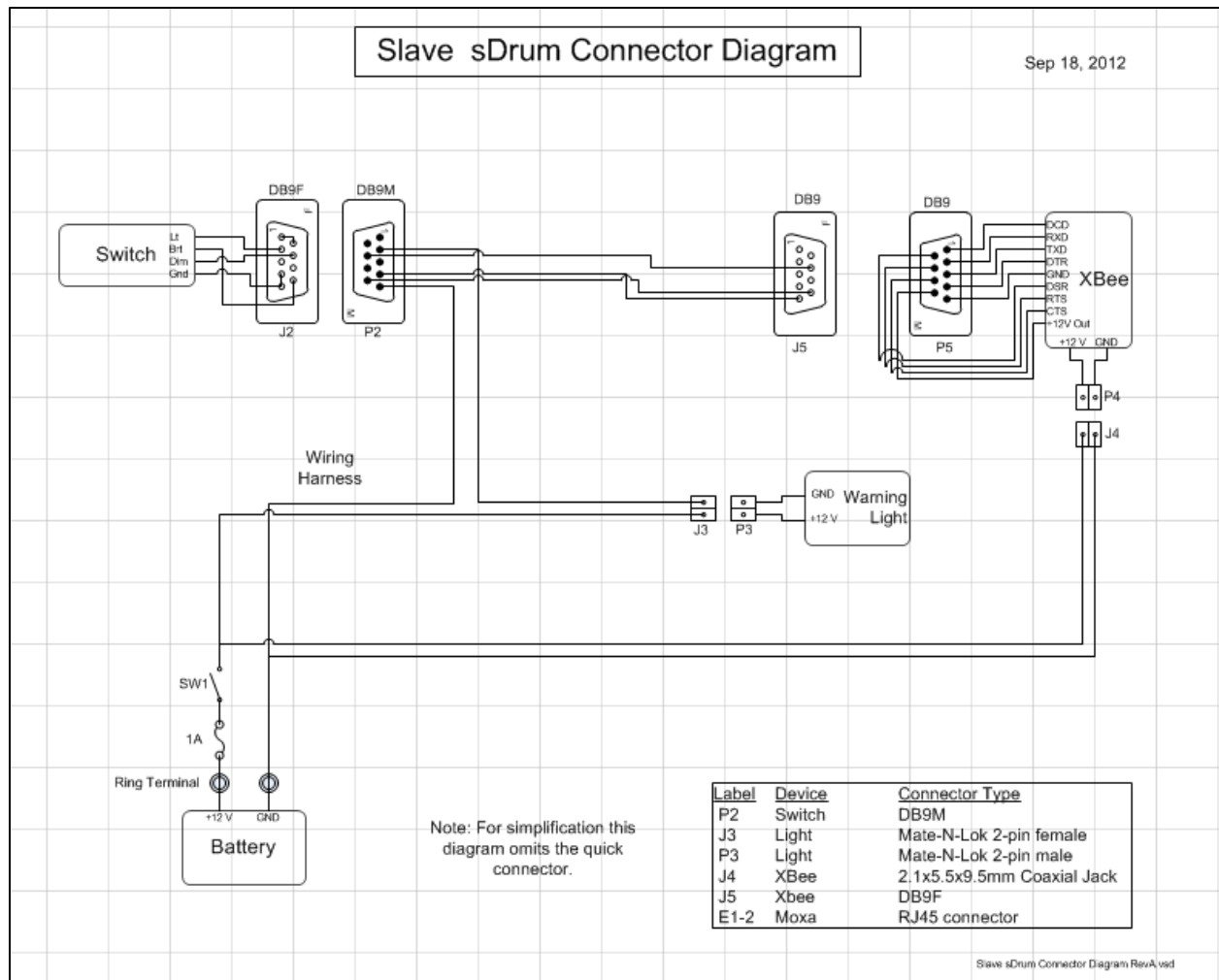
Figure 85: Slave Drum Connector Diagram
