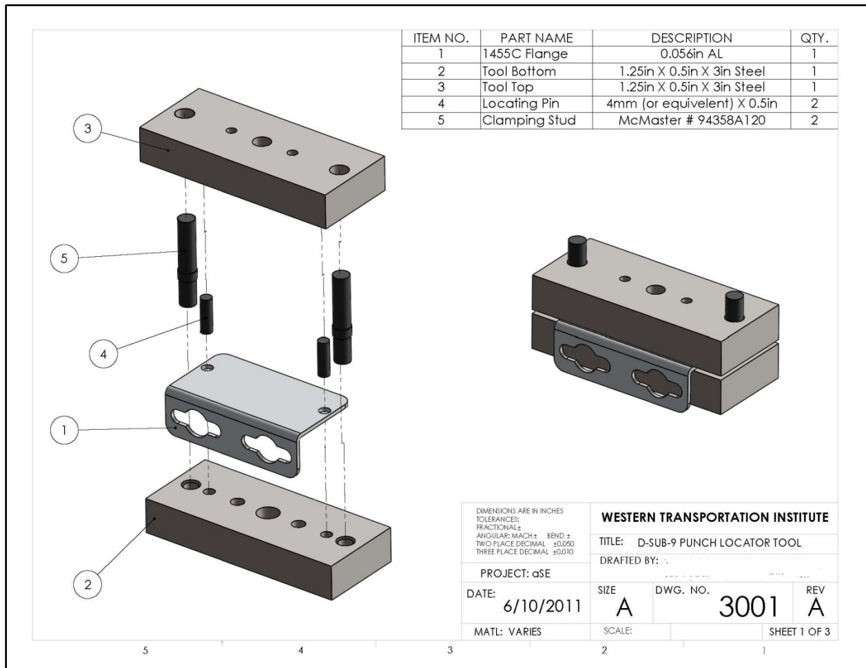
Figure 82: D-Sub-9 Punch Locator Tool
