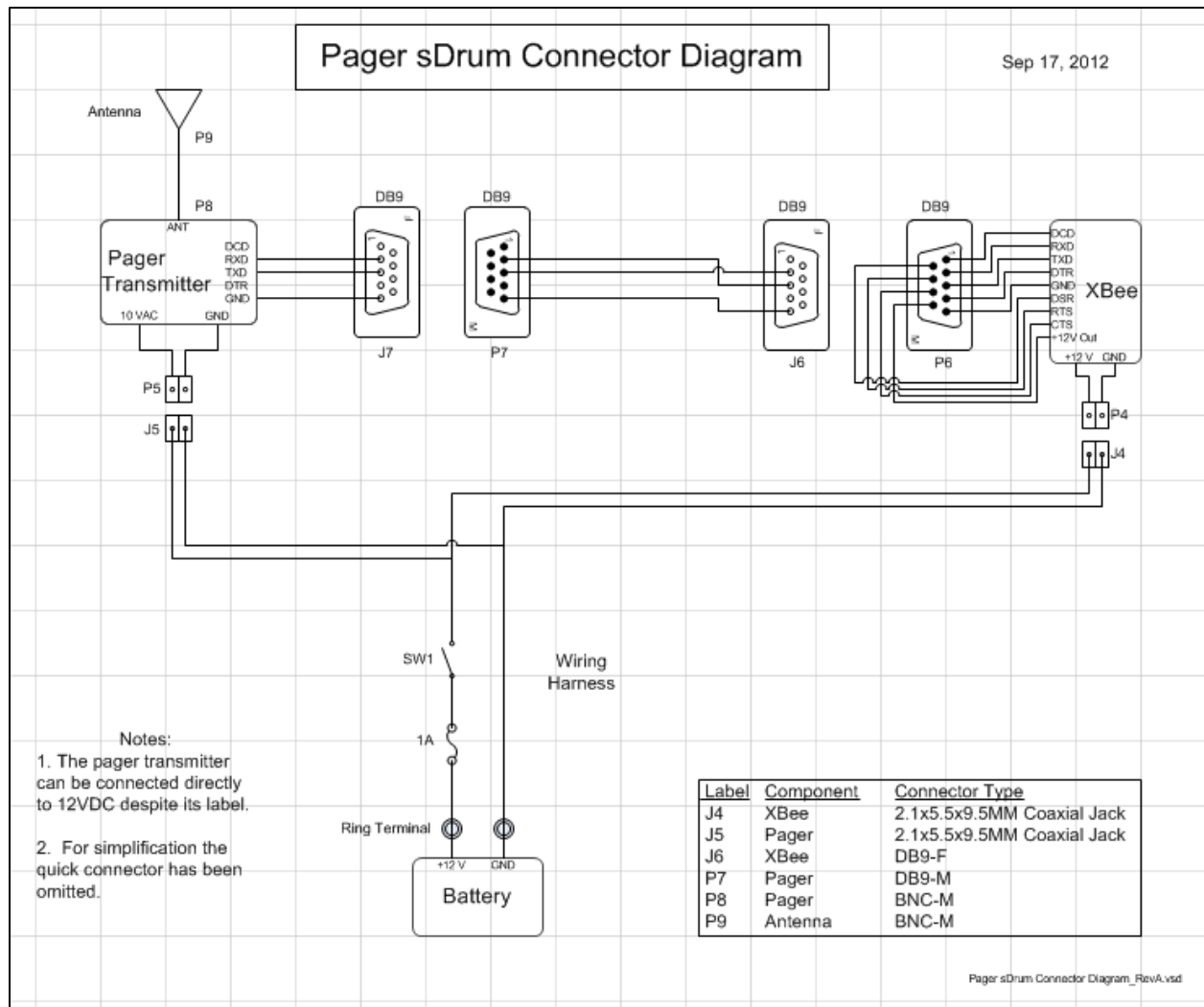
Figure 86: Pager Drum Connector Diagram
