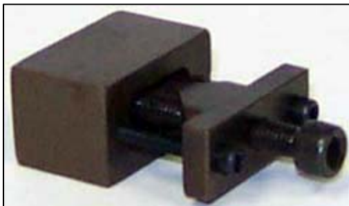
Figure 83: DB9 D-Sub Punch - Image Courtesy of Challenge Tool
