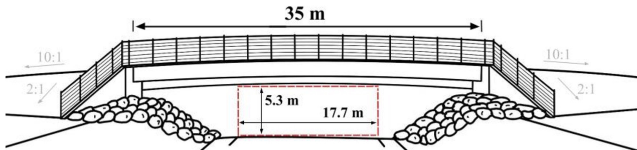
Figure 16: Elevation view of the US-97 wildlife overpass. Not Drawn to scale
