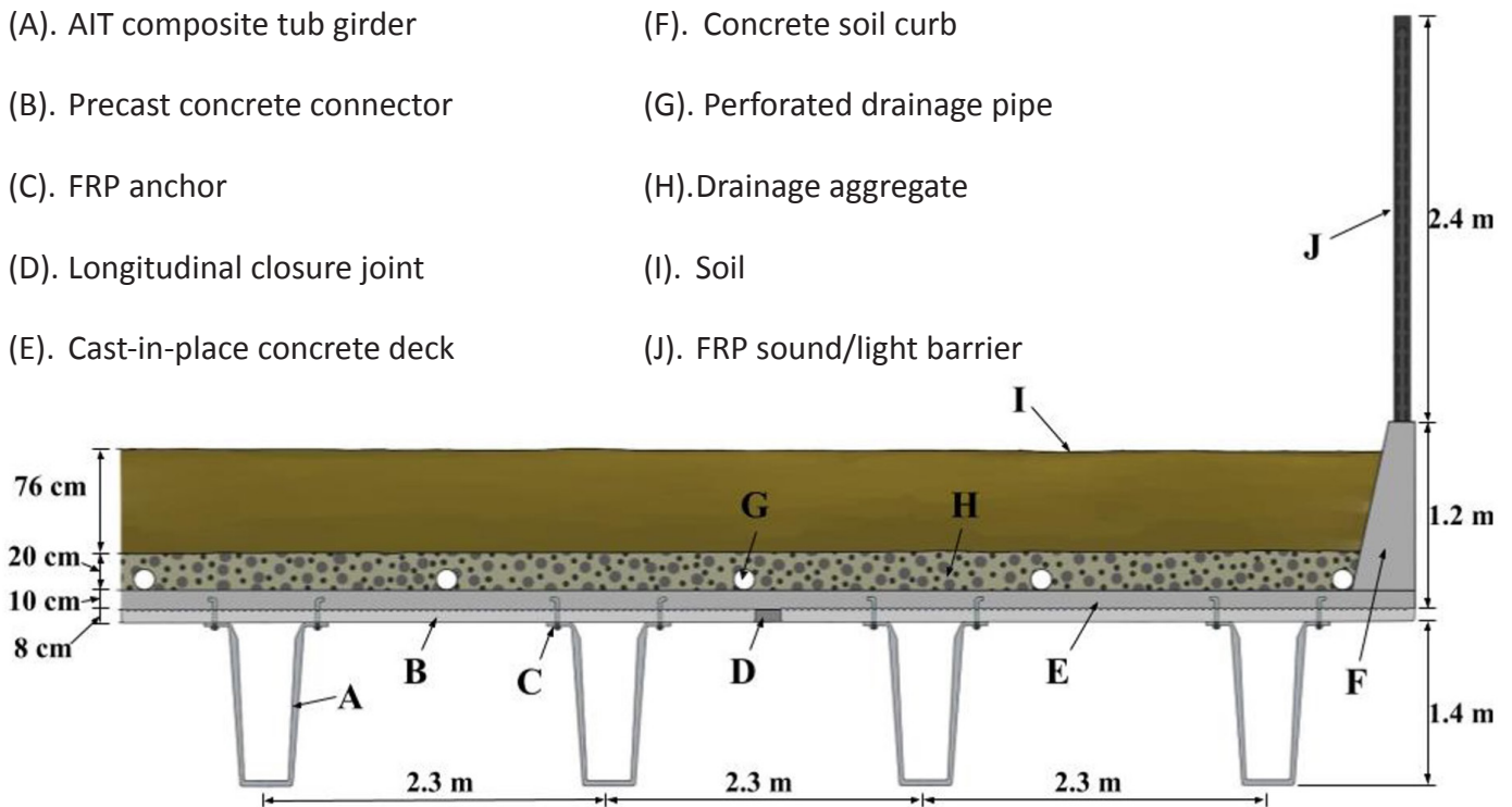
Figure 18: Cross section of the wildlife overpass showing the layout of the girders, concrete deck, soil, drainage, and barriers on the bridge span in meters (m). Not drawn to scale
