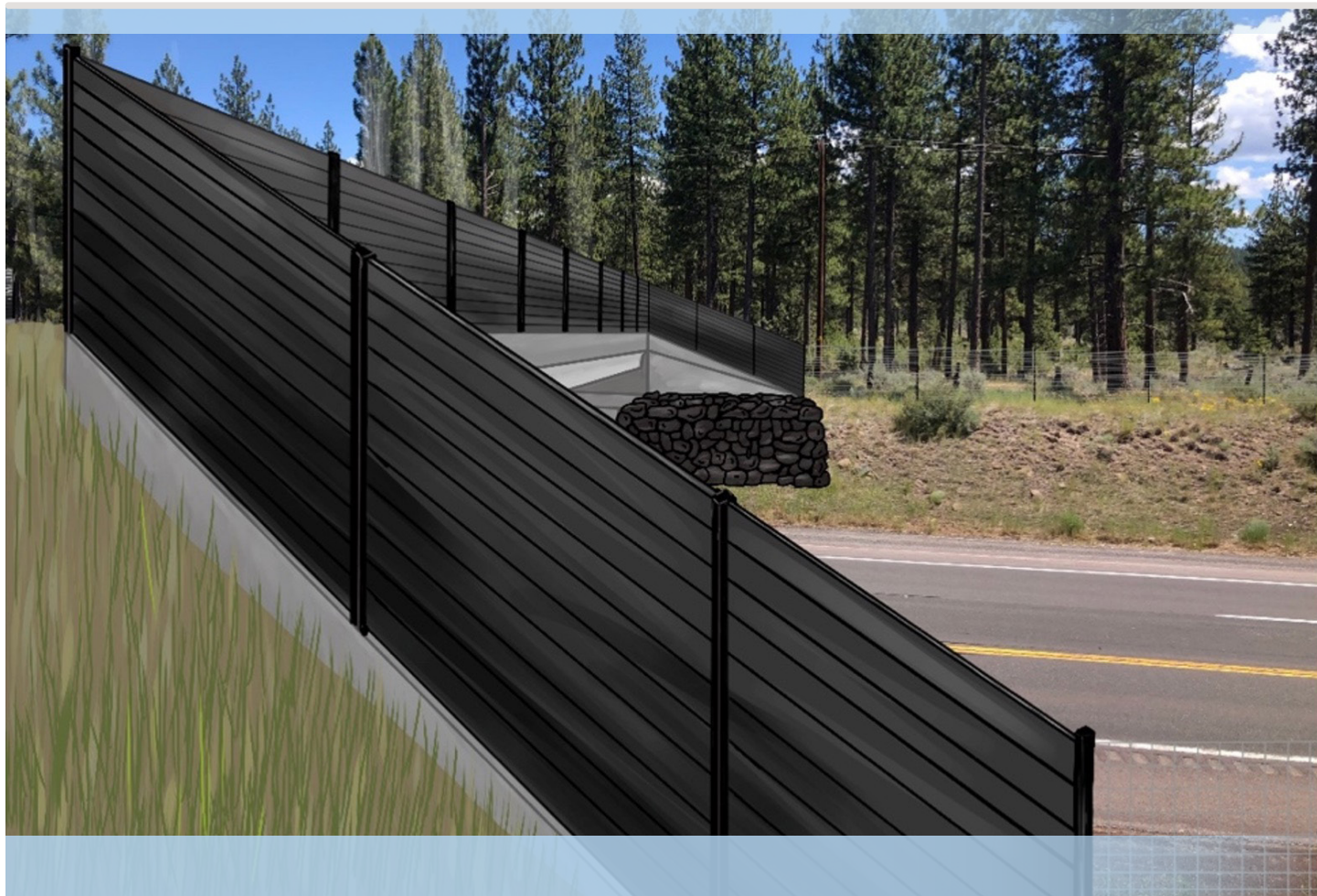
Figure 19: Rendering of a recycled-plastic sound and light barrier installed on top of the FRP overpass on US-97.
