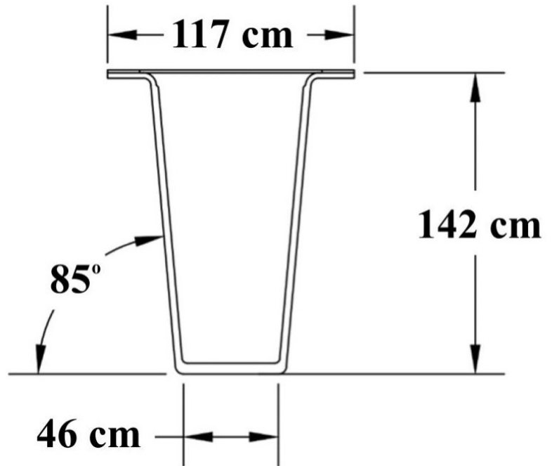
Figure 17: A photo and the dimensions in centimeters (cm) of the FRP or composite tub girder used to form the structure for the design of the wildlife overpass structure on US-97 in Siskiyou County, California (AIT Bridges). Not drawn to scale
